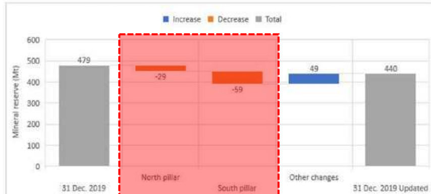
Figure 15.1 Hugo North changes to tonnage in the Probable Mineral Reserve
